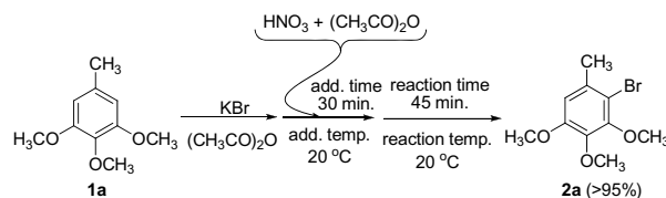
Scheme 1. An efficient high yielding bromination process. 11
